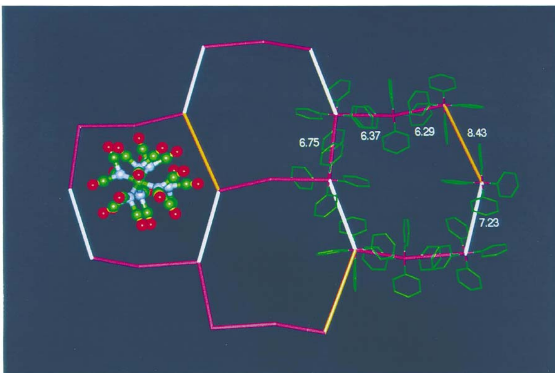
Fig. 5 Simplification of the crystal structure of [\text{Ph}_4\text{P}^+]_3[\text{CrE}_7(\text{CO})_{21}]^{3-} [BEJBOH]. Purple rods signify 6PE, orange rods are P4PE, and the white rods are asymmetric 4PE. This view of the P4PE at 8.43 Å illustrates well the offset-face-to-face and two edge-to-face \text{Ph}\cdots\text{Ph} interactions characteristic of P4PE. Note that the cation involved in the 6PE identified as 6.37, 6.29 Å is folded out of the cation layer, and that this occurs in such a way that the sheet of cations is corrugated left-right across the figure. The calculated energies of the embraces (identified by their \text{P}\cdots\text{P} distances) are given in \text{kcal mol}^{-1} per \{\text{Ph}_4\} set, and in square brackets per \{\text{Ph}_2\text{P}\}_2 set: 6PE at 6.29 Å, -8.9 [ -5.9 ]; 6PE at 6.37 Å, -6.7 [ -3.3 ]; 6PE at 6.75 Å, -4.8 [ -1.9 ]; 4PE at 7.23 Å, -5.2 [ -2.6 ]; P4PE at 8.43 Å, -4.1 [ -1.0 ] \text{kcal mol}^{-1} .
