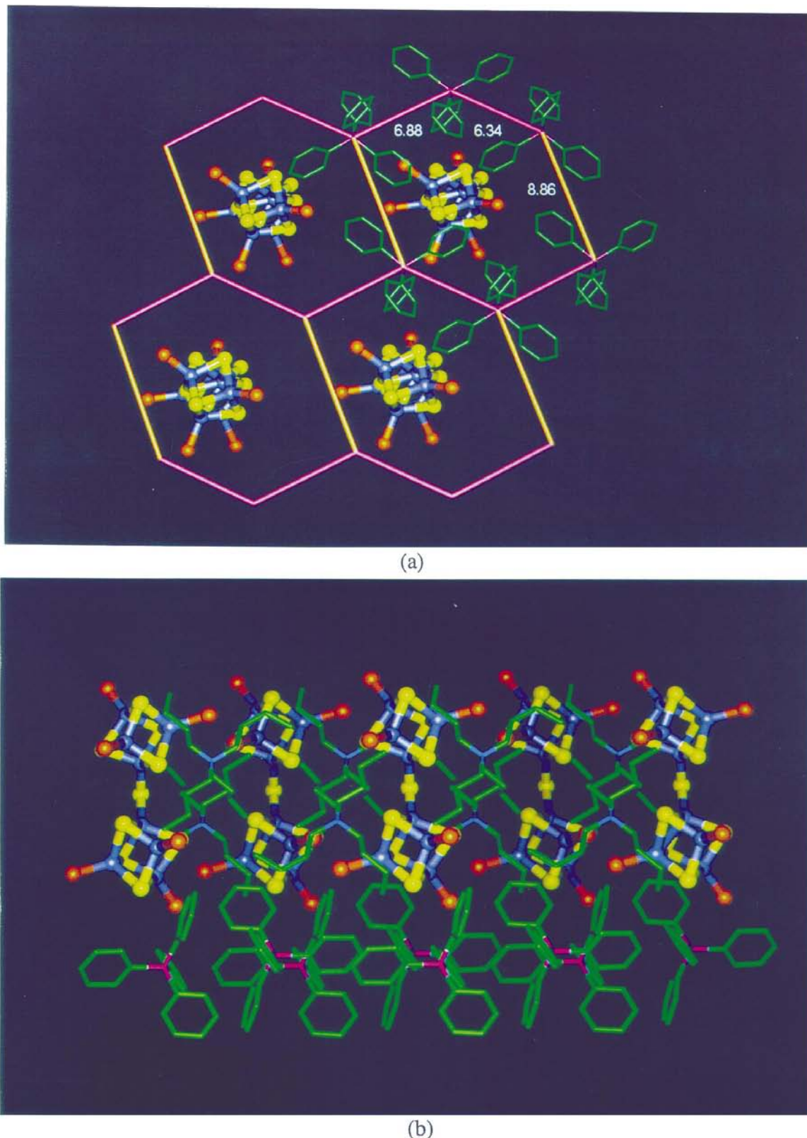
Fig. 2 Representations of the crystal structure of [\text{Ph}_4\text{P}^+]_2[\text{Bu}_4\text{N}^+]_2[\text{Fe}_8\text{S}_9\text{Cl}_6]^{4-} [JEGBAY]. (a) View of the hexagonal ZZI6PE/P4PE layer of \text{Ph}_4\text{P}^+ cations, and the locations of the anions under the hexagons. (b) Side view of the layered structure, showing the segregated layer of \text{Ph}_4\text{P}^+ cations, with the \text{Bu}_4\text{N}^+ cations interspersed in the layer of anions.
